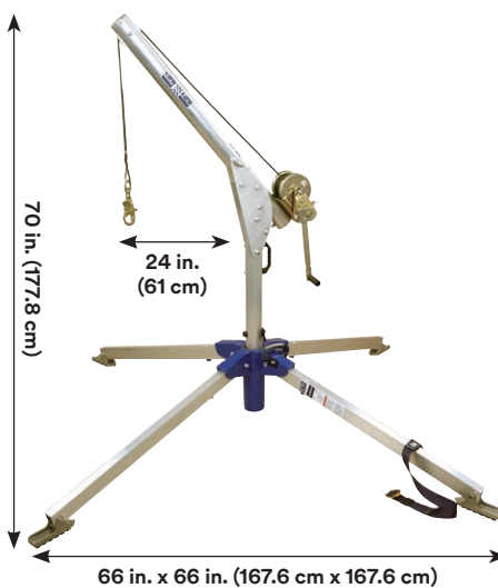
8302500 2-piece rescue davit system with folding base and arm, and 50 ft. (15.2 m) synthetic rope winch. Designed for rescue, retrieval, and descent applications only. Weight: 76.2 lbs. (34.6 kg)
