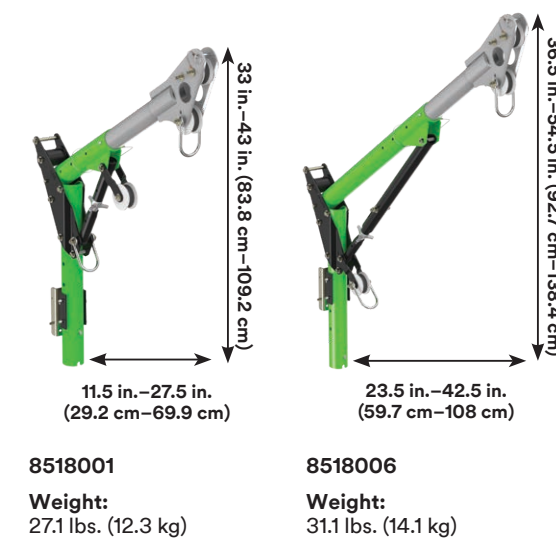
(Includes winch mount bracket) Combine these adjustable offset upper davit masts with up to two lower mast extensions to increase the davit height. Consult the compatibility charts.
